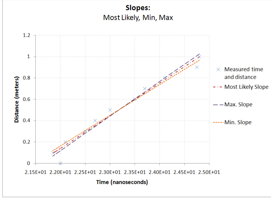
Figure 1 – Plot of measured times vs. distance (in m) from meter stick reading of 0.7m. The best, minimum and maximum slopes are also shown.
