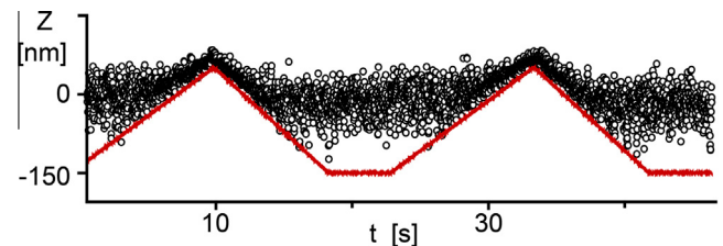
Fig. 4.2. Referencing separations between substrate and probe surfaces to the equilibrium position in the trap. When levitated above a surface in a trap, the procedure for determining the relative distance between the probe and substrate surfaces involves a programmed initialization cycle of up-down movement of the piezo stage, which pushes the probe up/down relative to the trap center. Matching the piezo-stage trajectory (red line in Fig. 4.2) to the indented profile of the Brownian height fluctuations (black circles) provides the bare height reference for the substrate surface relative to the trap center. The height referencing enables subsequent changes in surface separation to be defined relative to any piezo trajectory.
