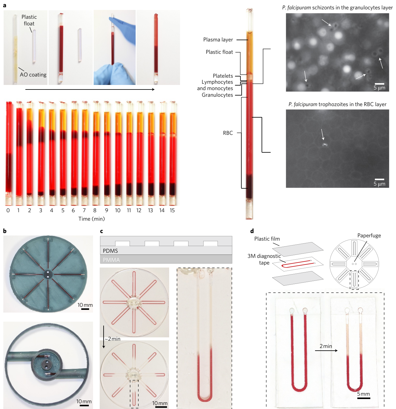
Figure 4 | Paperfuge applications and design landscape. a , QBC for malaria diagnosis. Top four panels: commercial QBC capillary (coated with acridine orange (AO) dye) and solid cylindrical float utilized on the paperfuge to achieve density-based stratification of blood components. Bottom: snapshots of separation over time; at t = 0 , the float is inserted into the top of the capillary; as soon as spinning commences, the float settles to the bottom. Over a period of 15 min, it rises to the plasma/RBC interface due to the difference in density, expanding the buffy-coat region. Right: using P. falciparum -infected blood, the parasite is rapidly visualized using a fluorescent microscope in specific density layers. b , 3D-printed devices. Lightweight polymeric materials can be rapidly printed for generating functional low-cost 3D-fuges. The two prototypes shown achieved speeds of approximately 10,000 r.p.m. and weighed <20 g. c , Using soft lithography, PDMS devices were fabricated to exploit centrifugal microfluidics. This PDMS-fuge was spun at 15,000 r.p.m., and plasma was separated in 2 min from 10 \mu l of blood. d , Plastic-tape microfluidics. Schematic showing two-dimensional 'slides' constructed using 3M diagnostic tape that can easily be attached to a paperfuge. A two-dimensional slide with a U-shaped channel showed plasma separation from 15 \mu l whole blood in 2 min.
