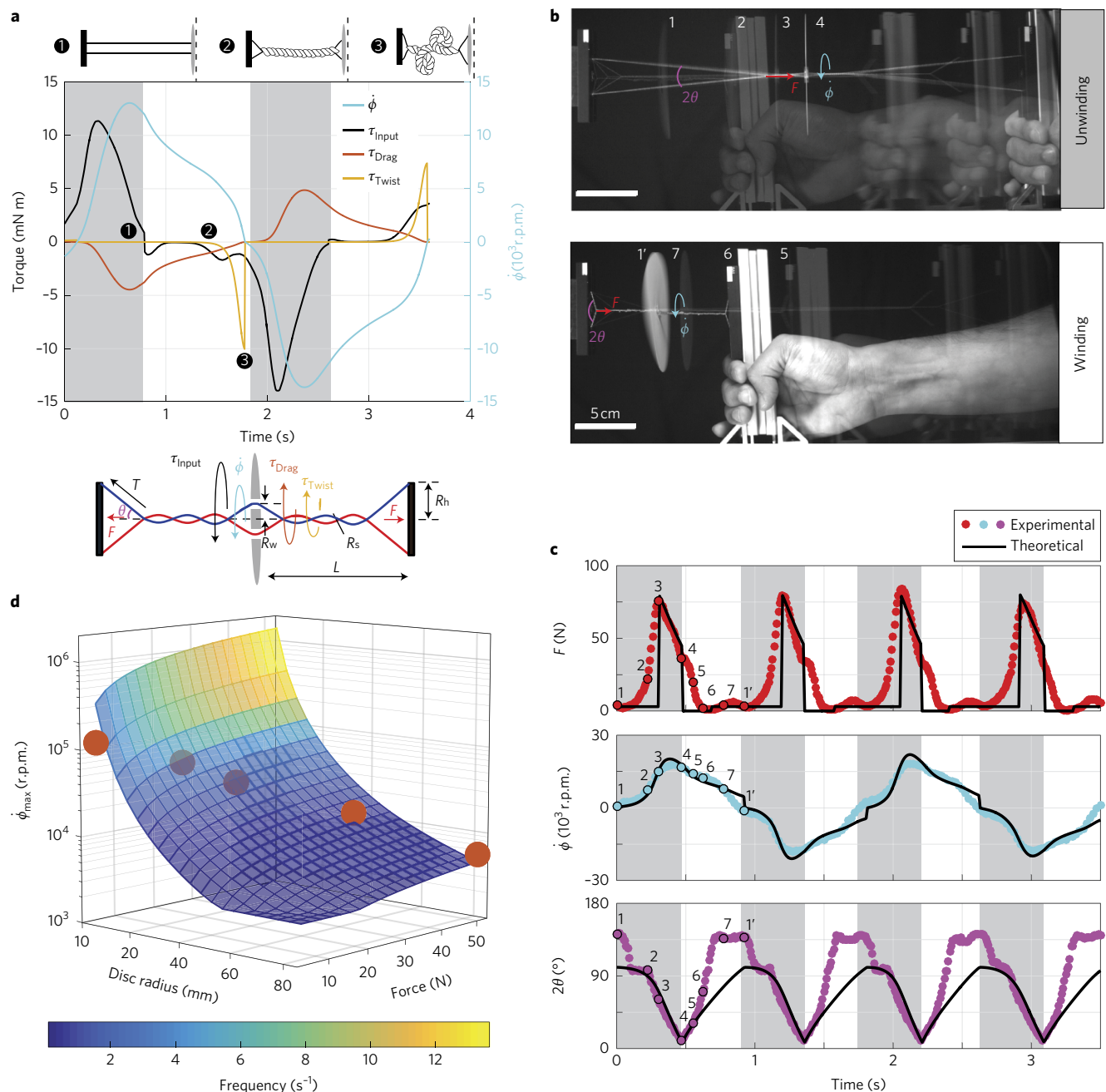
Figure 2 | Validation of the theoretical model with experiments. a , Numerical solution of equation (1) (Supplementary information), highlighting the contributions of different torque components. Schematics illustrate the coiling states (top) and the force–body diagram (bottom) of the paperfuge. b , Top: image of four superimposed snapshots (1–4) of the paperfuge during the ‘unwinding phase’, when F is applied, unwinding the coiled strings and accelerating the paperfuge to its maximum rotational speed (methods in Supplementary Information and Supplementary Video 4). Bottom: four superimposed snapshots (5–1’) showing the ‘winding phase’, when F falls to zero and the inertia of the disc causes re-winding of the strings. c , Synchronized time series plots of: force, F (top); \dot{\phi} of the disc (middle); and 2\theta of the strings (bottom). The coloured circles denote experimental data and the continuous black lines denote the theoretical predictions, which are in good agreement. When F is approximately zero, low string tension causes the strings to slacken, assuming a geometry outside the scope of our model and causing a systematic underprediction in \theta . d , The five experimental data points ( R_d of 5, 12.5, 25, 50 and 85 mm) along with a set of force-varying data (Supplementary Fig. 5) are used to tune the parameters of our model.
