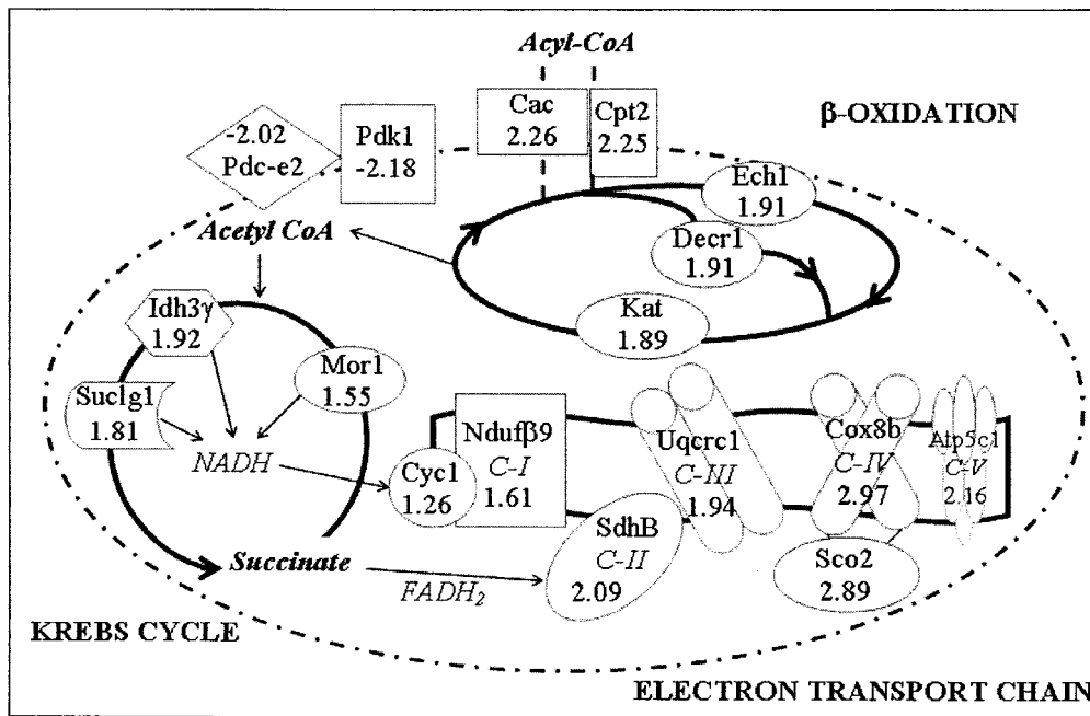
FIG. 2. Metabolic pathways altered in mouse plin -/- WAT: \beta -oxidation, Krebs cycle, and electron transport chain. Fold changes in transcript levels are listed beneath the gene symbols. Decr1, 2,4-dienoyl CoA reductase 1; Ech1, enoyl CoA hydratase 1; Kat, acetyl-CoA acyltransferase; Pdc-e2, dihydroliipoamide S-acetyltransferase; Idh3 \gamma , isocitrate dehydrogenase [NAD] \gamma ; Suc1g1, succinate-CoA ligase GDP-forming \alpha ; Mor1, malate dehydrogenase mitochondrial; Nduf \beta 9, NADH dehydrogenase (ubiquinone) 1 \beta 9; SdhB, succinate dehydrogenase complex, B-Ip; Uqcrc1, ubiquinol-cytochrome C reductase 1; Cyc1, cytochrome C-1; Cox8b, cytochrome C oxidase polypeptide VIIIb; Sco2, cytochrome C oxidase assembly protein 2; Atp5c1, ATP synthase, H + -transporting, F1 \gamma 1. Substrates are shown in italics.
