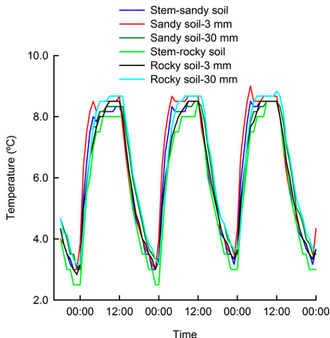
Fig. 7. Temperatures recorded for soil and plants in large containers in a growth chamber (8°C day/3°C night). Thermal sensors were embedded in plants in sandy soil (dark-blue line), in sandy soil at 3 mm (red line) and at 30 mm deep (dark-green line), in plants embedded in rocky soil (light-green line), and in rocky soil at 3 mm (black line) and at 30 mm (light-blue line). N = 3 for each condition; SE (not shown for sake of legibility) was less than 2% of the mean in all cases.
