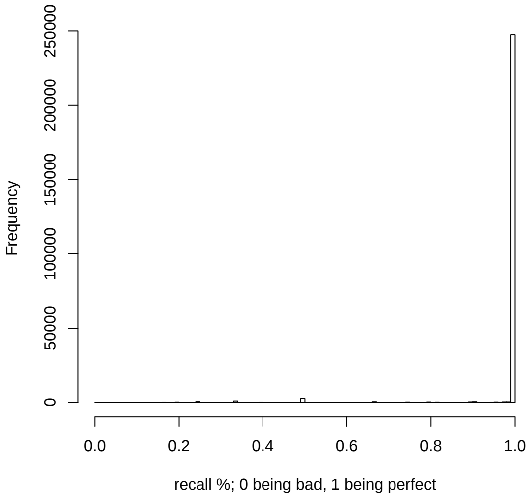
Frequency of families' recall % (excluding non hit families)
