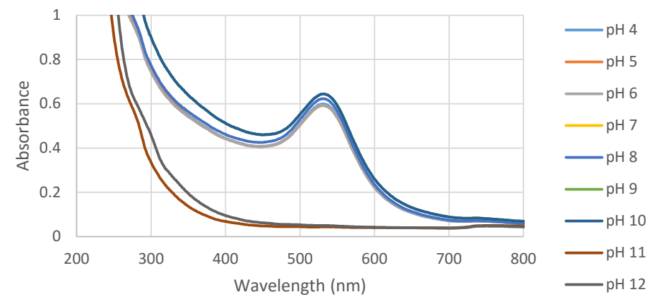
UV-Vis; [Gold NP]=0.25 mM, [Fructose]=0.0625 mM, No Correction
