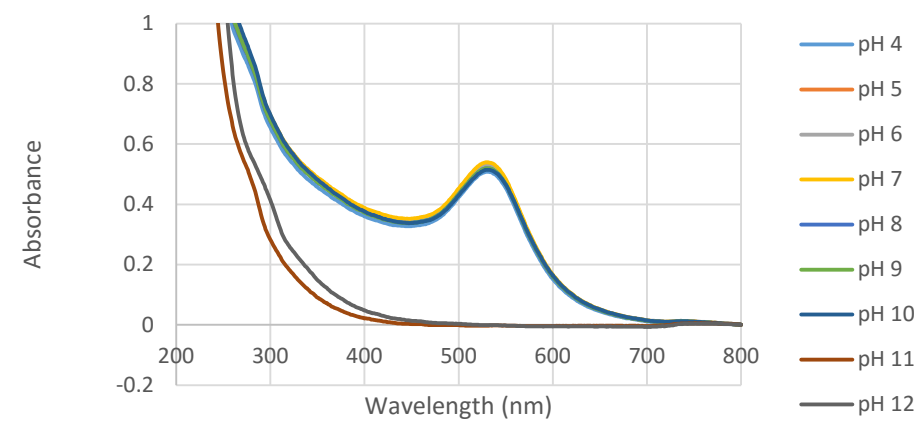
UV-Vis; [Gold NP]=0.25 mM, [Fructose]=0 mM, Baseline Corrected
