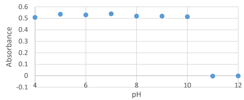
A(530), [Fructose]=0 mM, Baseline Corrected
