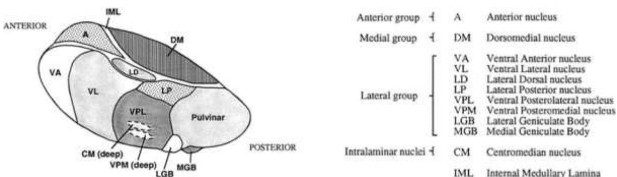
Figure 5.5 Thalamic Nuclei
